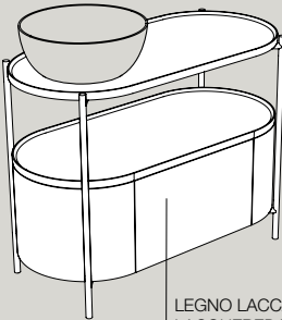
200S7607 struttura h 76 cm_frame h 76 cm 200M madia ovale_oval sideboard 200R ripiano_shelf 100x48xh93 cm
