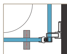
Detaliu A - plan pardoseala
